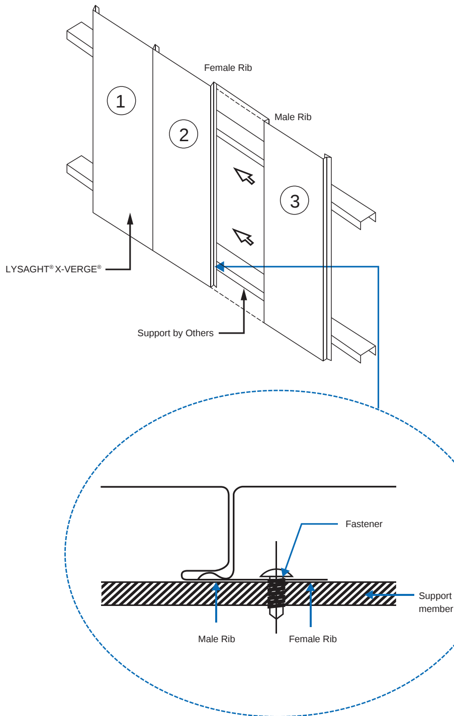
Figure 2.0: Fastening to support of LYSAGHT® X-VERGE®
